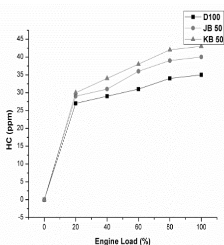
Fig. 4. Effect of engine load on hydrocarbon emission
