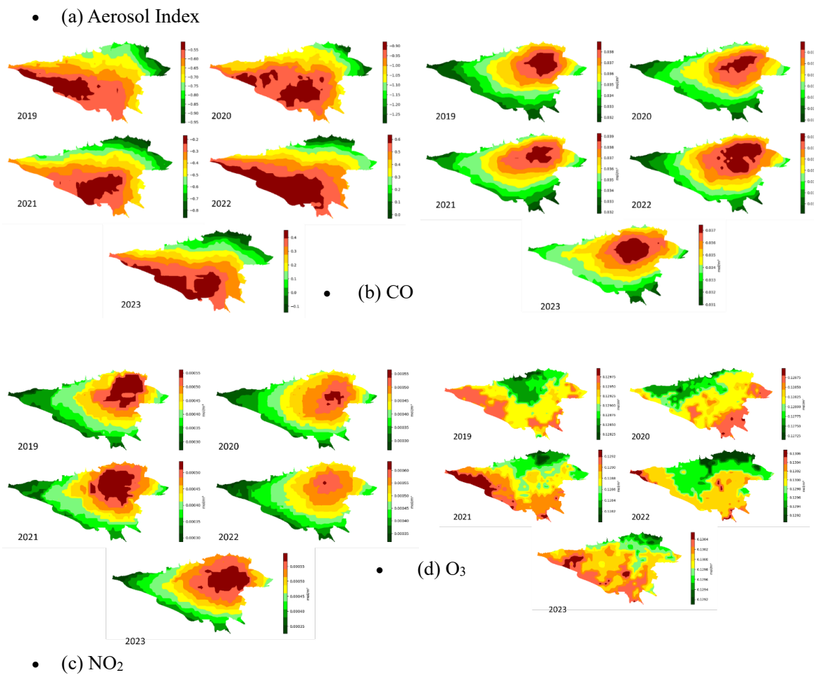
Fig. 3. Spatial distribution maps for aerosol index, CO, NO 2 , and O 3 .
