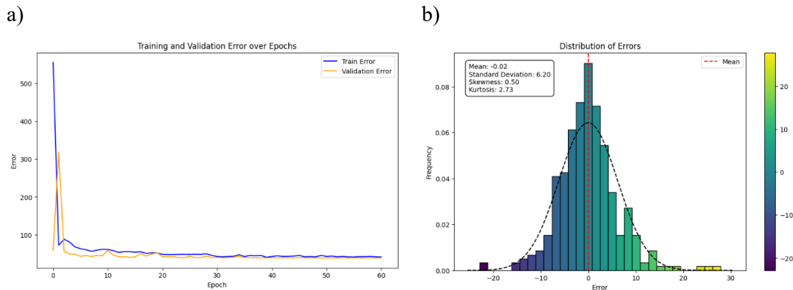
Fig. 4. a) Error versus epoch graph for training the neural network at the Tarbiat Modares station for the PM 2.5 pollutant. b) Histogram of error distribution at the Tarbiat Modares station for the PM 2.5 pollutant.
