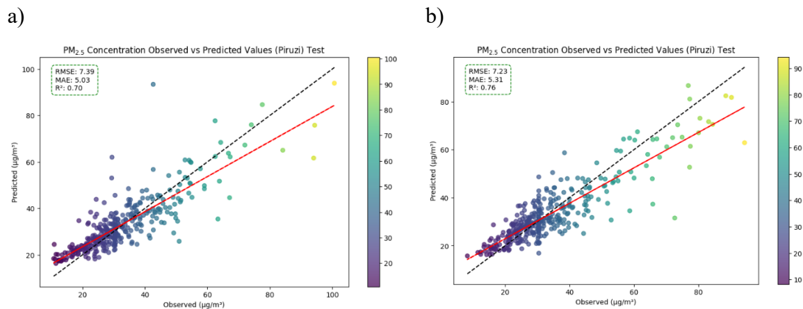
Fig. 5. a) Graph of observed versus predicted values for PM 2.5 at the Piruzi station using only ground-based data. b) Graph of observed versus predicted values for PM 2.5 at the Piruzi station using a combination of ground-based and satellite data.
