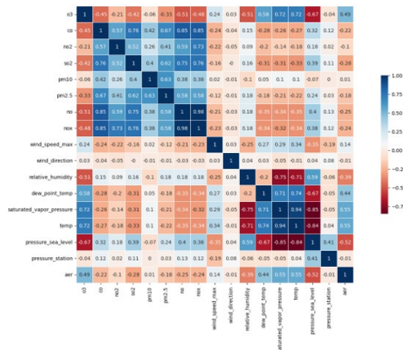
Fig. 2. Pearson's Correlation Matrix for Tarbiat Modares Station
