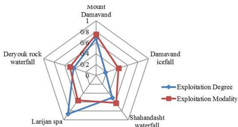
Fig. 4. Comparing the values for Exploitation Degree and Exploitation Quality of Geomorphological Landforms of Haraz Watershed
