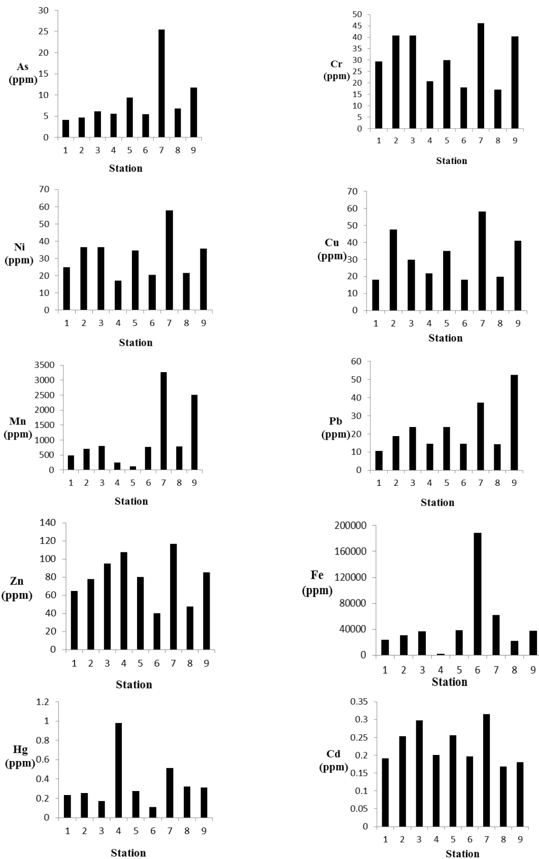
Fig. 2. Heavy metal distribution in different locations' sediments
