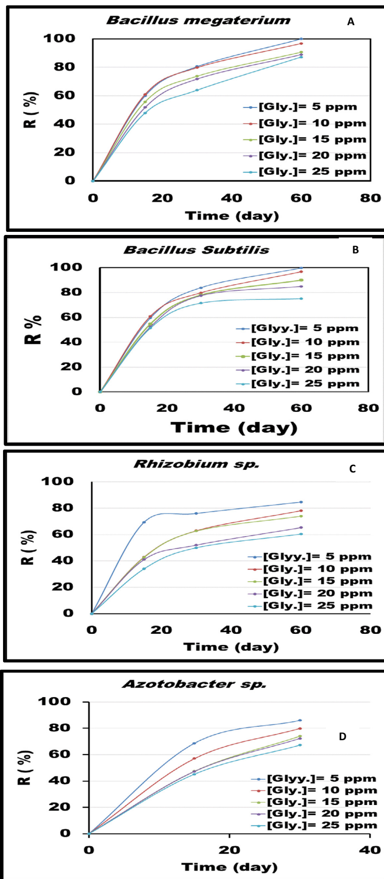
Fig. 3. The Removal Efficiency of Glyphosate Biodegradation using different bacterial.
