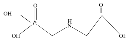
Fig. 2. The chemical formula of Glyphosate
