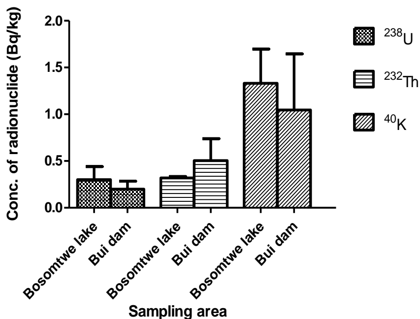
Fig. 5. Average activity concentrations of natural occurring radionuclides in ( ^{238}\text{U} , ^{232}\text{Th} , and ^{40}\text{K} )
