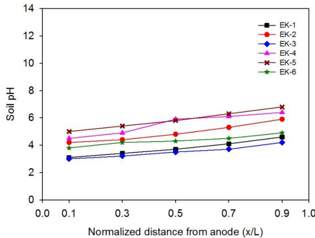
Fig. 2. Changes of pH in the soil with distance
